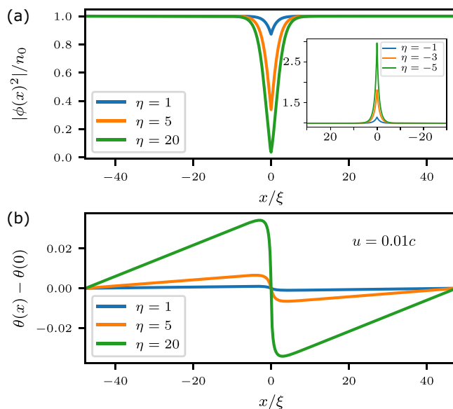
FIG. 1. Mean-field solution for different interactions and various couplings. All other parameters are as in Ref. [15], i.e., M/m = 0.47 , the peak density n_0 = 7/\mu\text{m} , and g_{\text{BB}} = 2.36 \times 10^{-37} \text{ Jm} . For the phase, we fixed u = 0.01c , which fixes the total momentum on the mean-field level.
