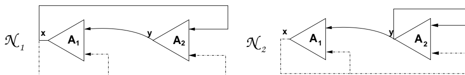
FIGURE 12. The networks \mathcal{N}_1 , \mathcal{N}_2 : equivalent 2 cell networks.
