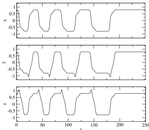
FIGURE 20. Time series x, y, z of (5.8) with f defined by (5.9), giving an attracting simple heteroclinic cycle. Note that there is a switching between two states that are both of from (x, x, x) , and a slowing down associated with approach the heteroclinic cycle.
