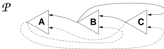
FIGURE 36. The network \mathcal{P} on \mathbf{S}_3 .
