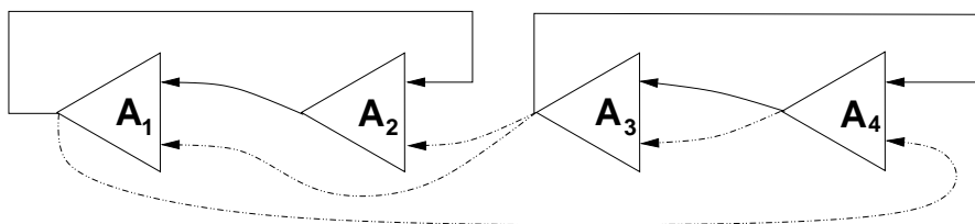
FIGURE 25. A network with one non-maximal synchrony class \{\mathbf{A}_1, \mathbf{A}_2\} in addition to maximal synchrony.
