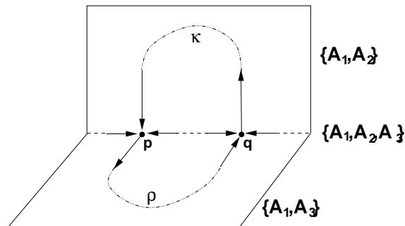
FIGURE 17. A simple heteroclinic cycle connecting \mathbf{p}, \mathbf{q} .
