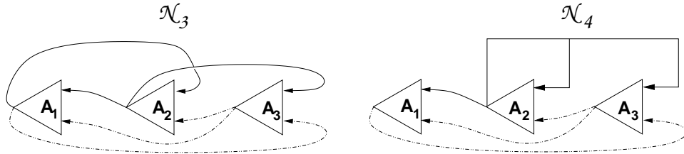
FIGURE 16. The two inequivalent networks with non-maximal synchrony classes \{\mathbf{A}_1, \mathbf{A}_2\} , \{\mathbf{A}_1, \mathbf{A}_3\} .
