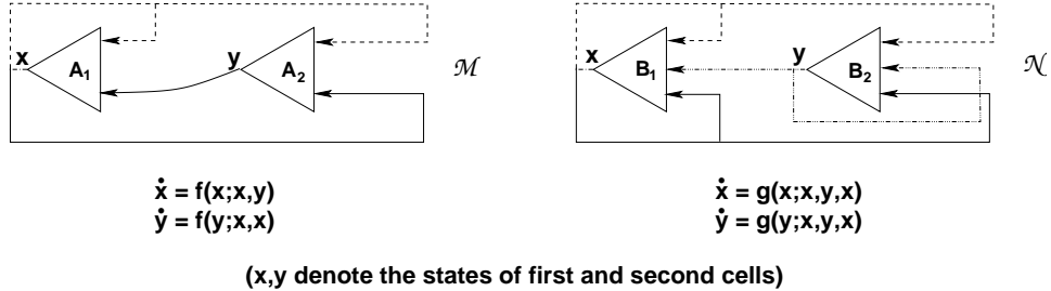
FIGURE 1. Dynamically equivalent networks; for any f that represents the cell dynamics of the network on the left, there is a g that gives precisely the same dynamics for the network on the right, and vice-versa.
