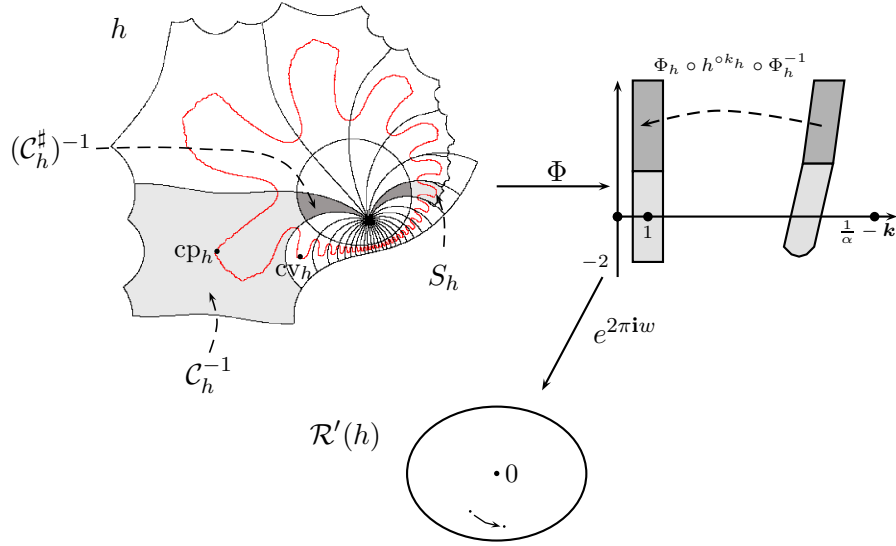
FIGURE 2. The figure shows the sets C_h, C_h^\sharp, \dots, C_h^{-k_h}, (C_h^\sharp)^{-k_h} , and the sector S_h . The induced map \Phi_h \circ h^{\circ k_h} \circ \Phi_h^{-1} projects via e^{2\pi i w} to a well-defined map \mathcal{R}(h) on a neighborhood of 0. The amoeba curve around 0 is a large number of iterates of cp_h under h .
