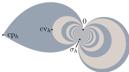
FIGURE 1. The domain \mathcal{P}_h and the special points associated to some h \in \mathcal{IS}_\alpha . The map \Phi_h sends each colored croissant to an infinite vertical strip of width one.
