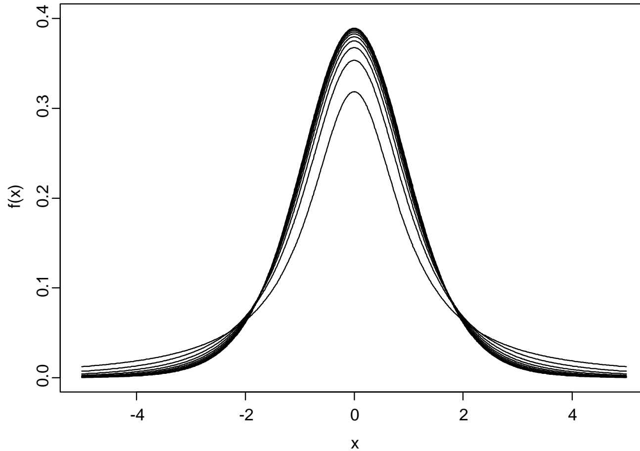
Student(n) pdf for n=1,...,10
