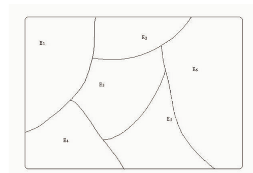
A partition of S
