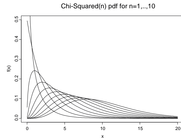
CHI-SQUARED PDF with n DEGREES OF FREEDOM
