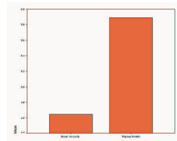
BAR PLOT
