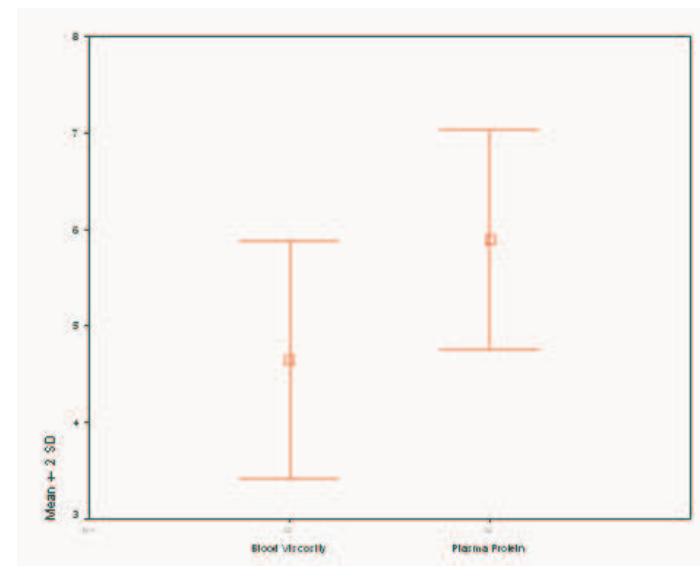
MEAN \pm 2 \times S.D.
