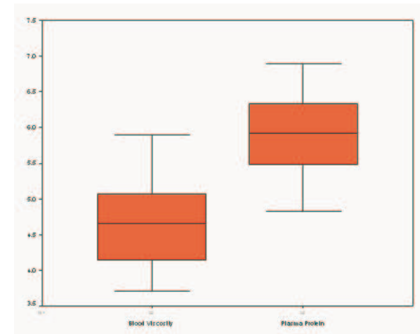
BOXPLOT for two groups of observations
