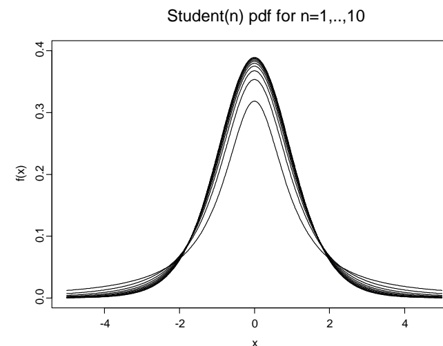
STUDENT-T PDF with n DEGREES OF FREEDOM
