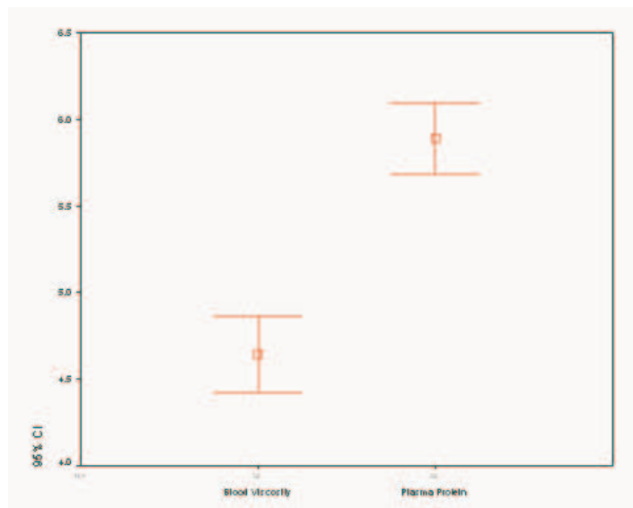
CONFIDENCE INTERVAL
