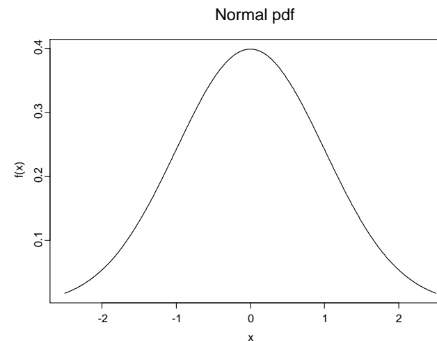
NORMAL PDF
