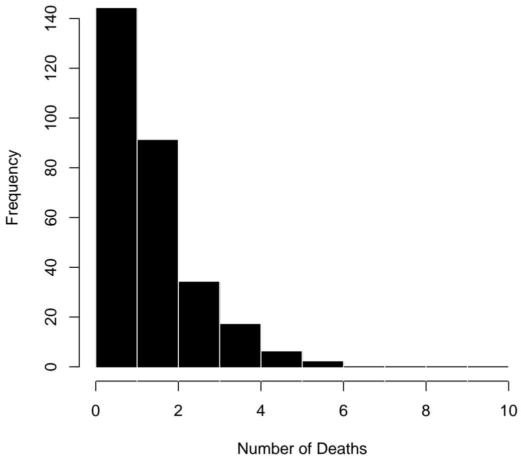
Histogram of Horsekicks Data
