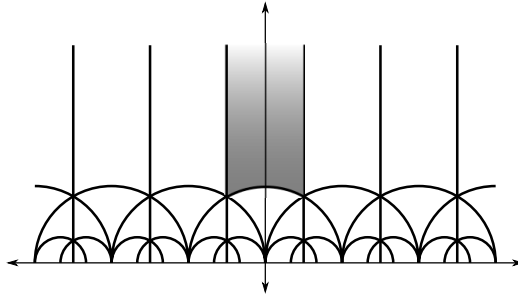
FIGURE 1. A fundamental domain for \mathrm{SL}_2(\mathbb{Z}) acting on \mathbb{H}^2
